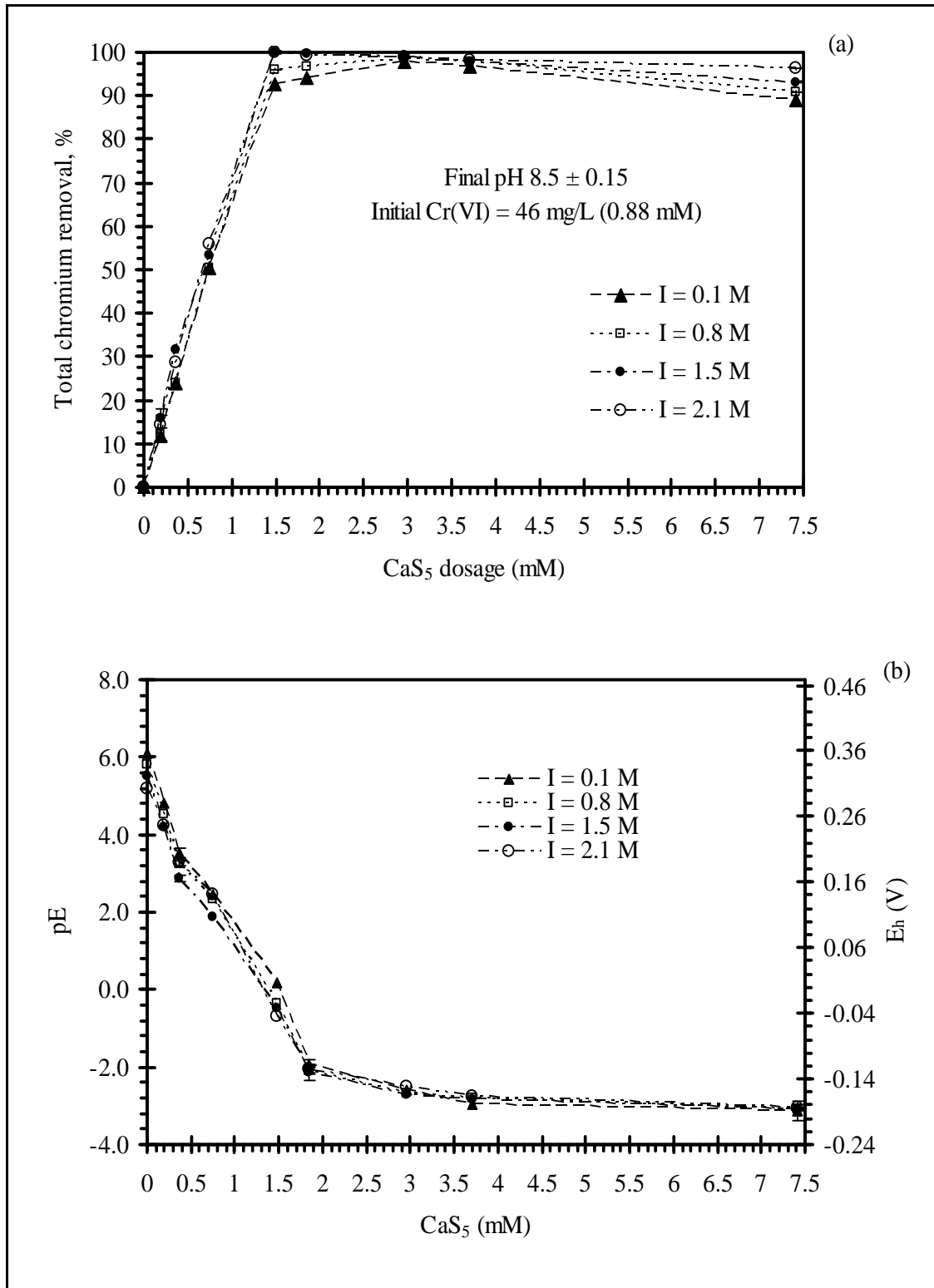
Figure 6.1a Chromium Removal Efficiency as a Function of CaS 5 Dosage and Different Ionic Strength Levels at a Constant Initial Cr(VI) Concentration of 46 mg/L (0.88 mM), pH of 8.5 ± 0.15, and Alkalinity of 5 g/L of CaCO 3 . Figure 6.1b Oxidation/Reduction Potential (E h ) and pE for Experimental Points Shown in Figure 6.1a
