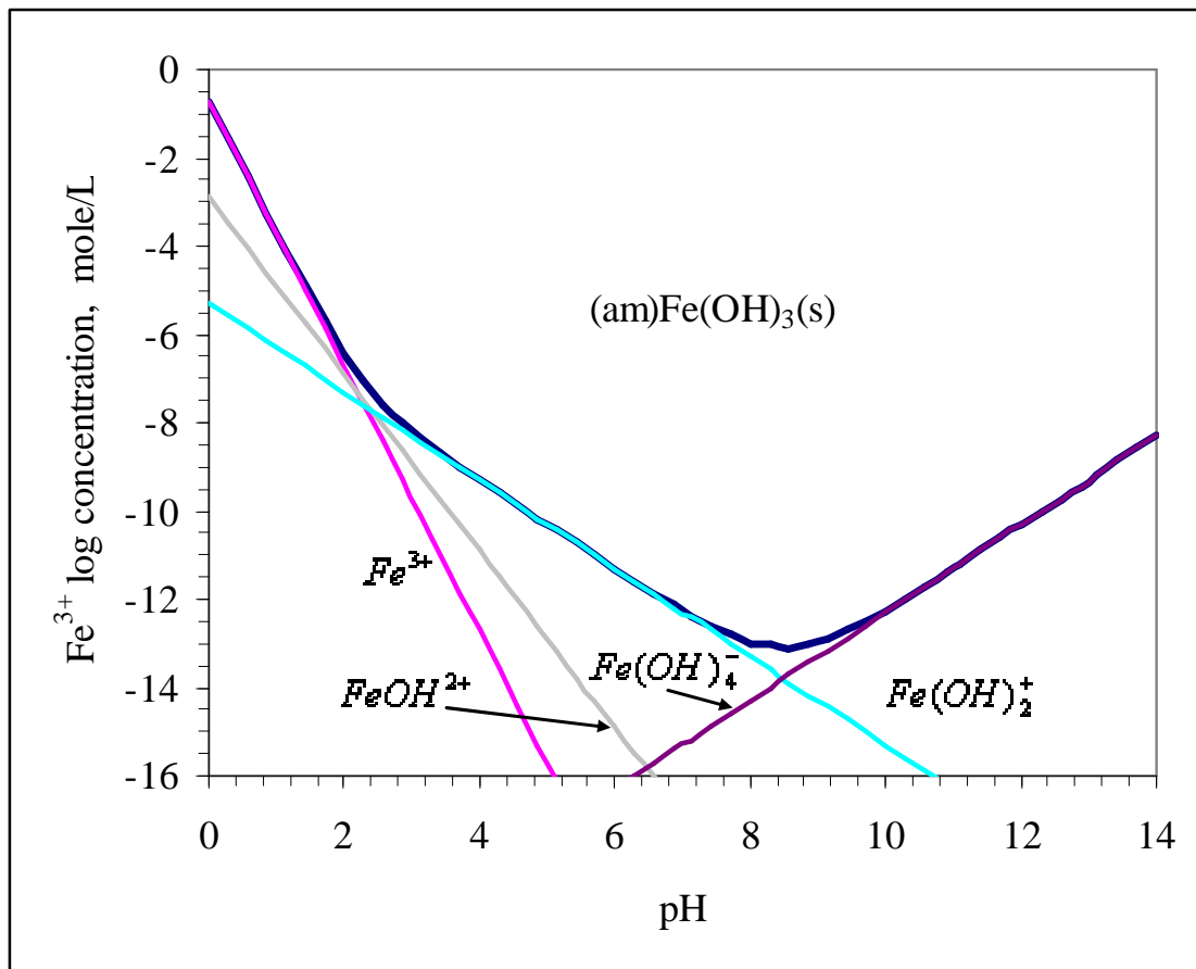
Figure 2.6 Computed Solubility of Precipitated \text{Fe}(\text{OH})_3 (S) (25°C, Initial Fe(III) = 56 g/L (1 M)) (MINEQL+ Was Utilized for the Computation, Schecher and Mcavoy, 2001)
