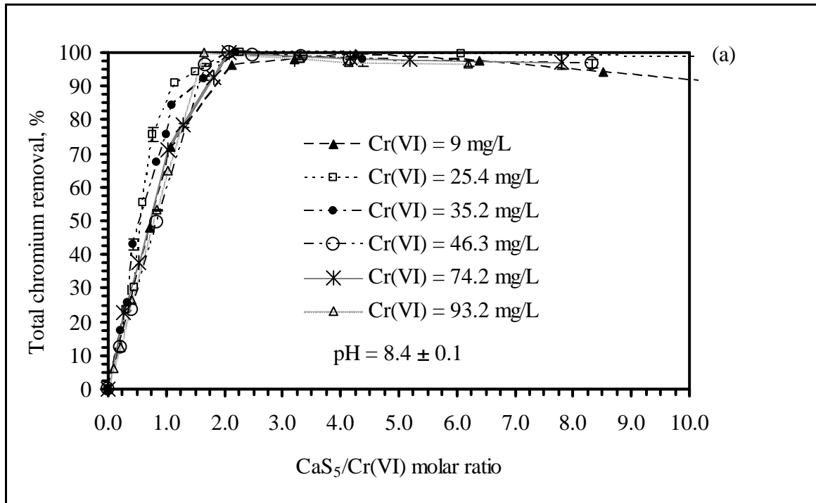
Figure 6.5 Total Chromium Removal as a Function of CaS 5 /Cr(VI) Molar Ratio and Different Initial Cr(VI) Concentrations for Brines with Ionic Strength of 0.8 M, Alkalinity of 5 g/L of CaCO 3 , and a Constant pH of 8.4 ± 0.1
