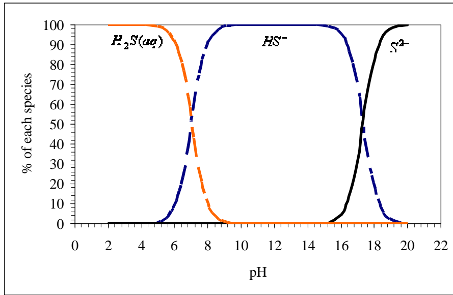
Figure 2.20 Computed Liquid-Phase Distributions of Ionic Species for H 2 S/HS - /S 2- System (MINEQL+ Was Utilized for the Computation, Schecher and Mcavoy, 2001)
